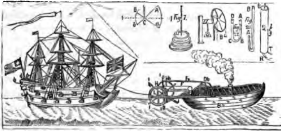
FIG. 66.—Hull's Steamboat, 1736.
